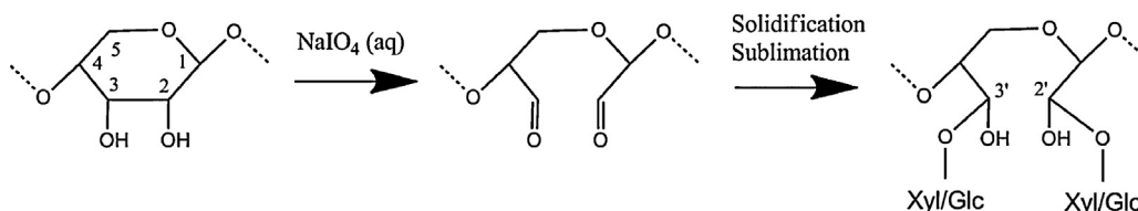
Fig. 2. Proposed reactions involved in cross-linking of xylan–cellulose nanocrystal composite hydrogels during freeze-casting.
