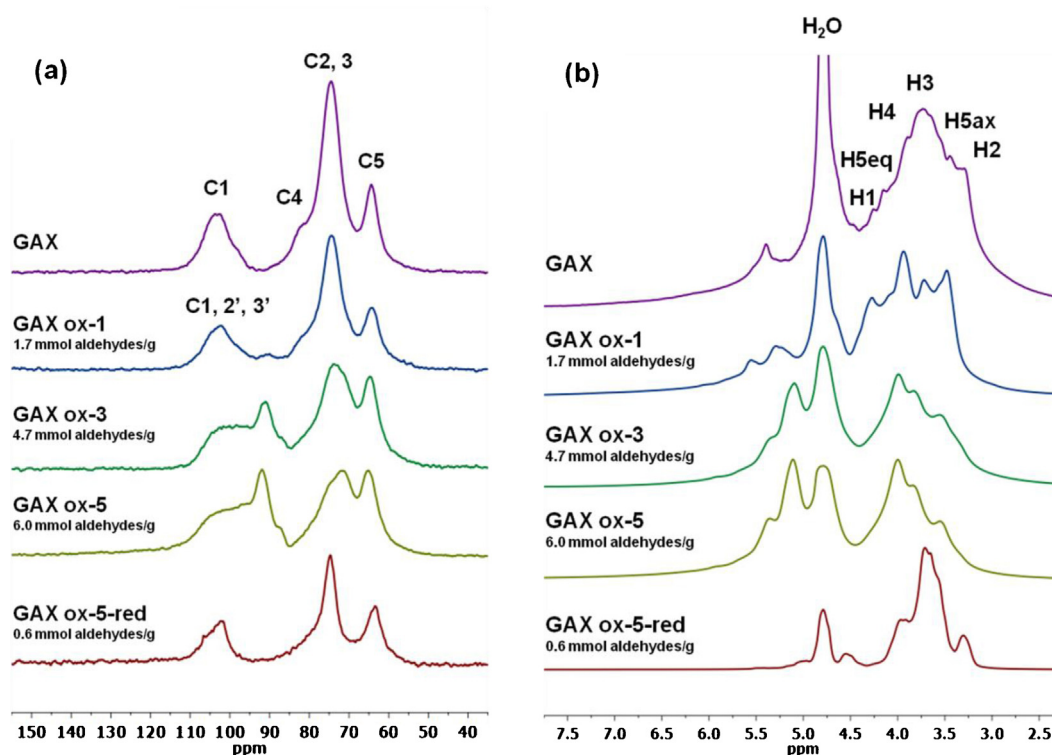
Fig. 4. ^{13}\text{C} (a) and ^1\text{H} (b) CP/MAS NMR spectra for freeze-dried reference xylan (GAX), oxidized xylns (GAX ox), and for a xylan sample first oxidized and then reduced by \text{NaBH}_4 (GAX ox-5-red). Cf. Fig. 2 for carbon numbering.
