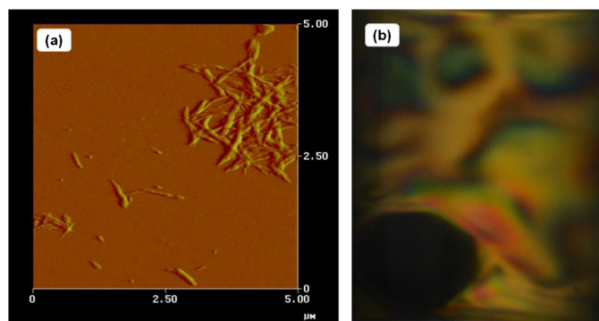
Fig. 3. (a) AFM image of obtained cellulose nanocrystals (CNCs). (b) Shear-induced birefringence of a 1% (w/w) CNC suspension viewed between crossed polars.
