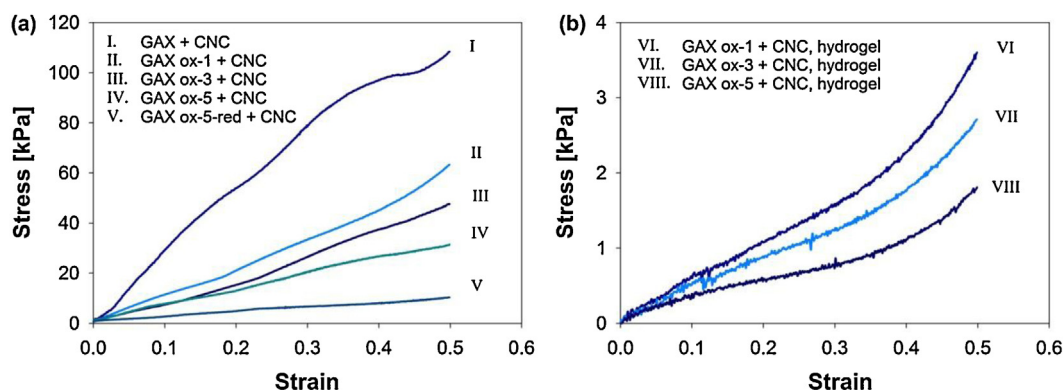
Fig. 7. Stress-strain curves of freeze-cast xylan-cellulose nanocrystal foams (a) and hydrogels (b).
