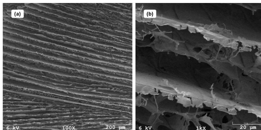
Fig. 6. Cross-section of an ice-templated, unidirectionally solidified, foam containing oxidized xylan (6 mmol aldehydes/g) and cellulose nanocrystals (20%). SEM magnification: (a) 100 \times (b) 1000 \times .
